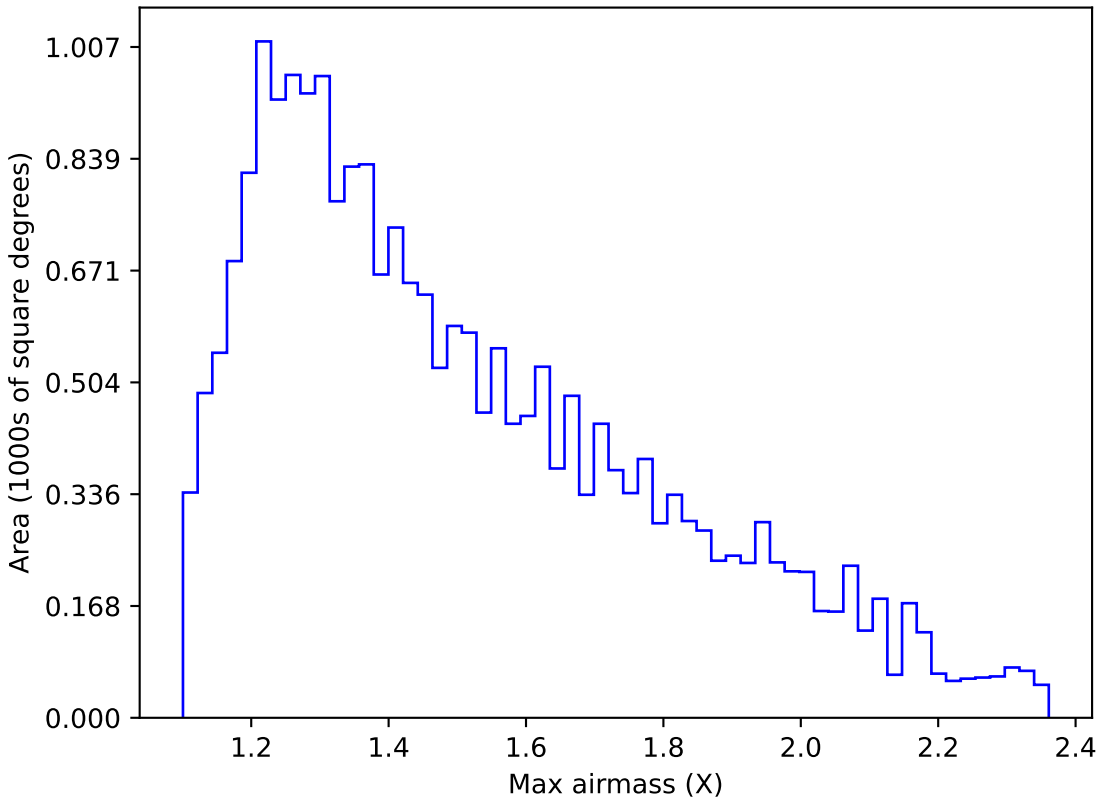
ddf_loaded_half_fl4_v3.4_10yrs Yr 1 u band: Max airmass
