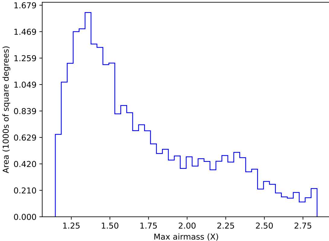
ddf_loaded_half_fl4_v3.4_10yrs Yr 1 i band: Max airmass
