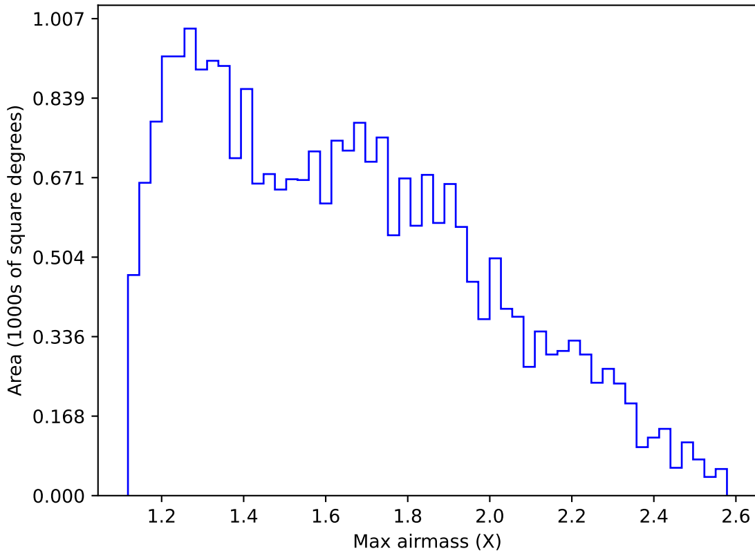
ddf_loaded_half_f14_v3.4_10yrs Yr 1 g band: Max airmass
