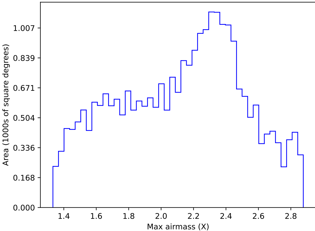
ddf_loaded_half_fl4_v3.4_10yrs Yr 1 all bands: Max airmass
