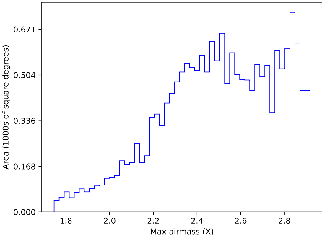
ddf_loaded_half_fl4_v3.4_10yrs WFD z band: Max airmass
