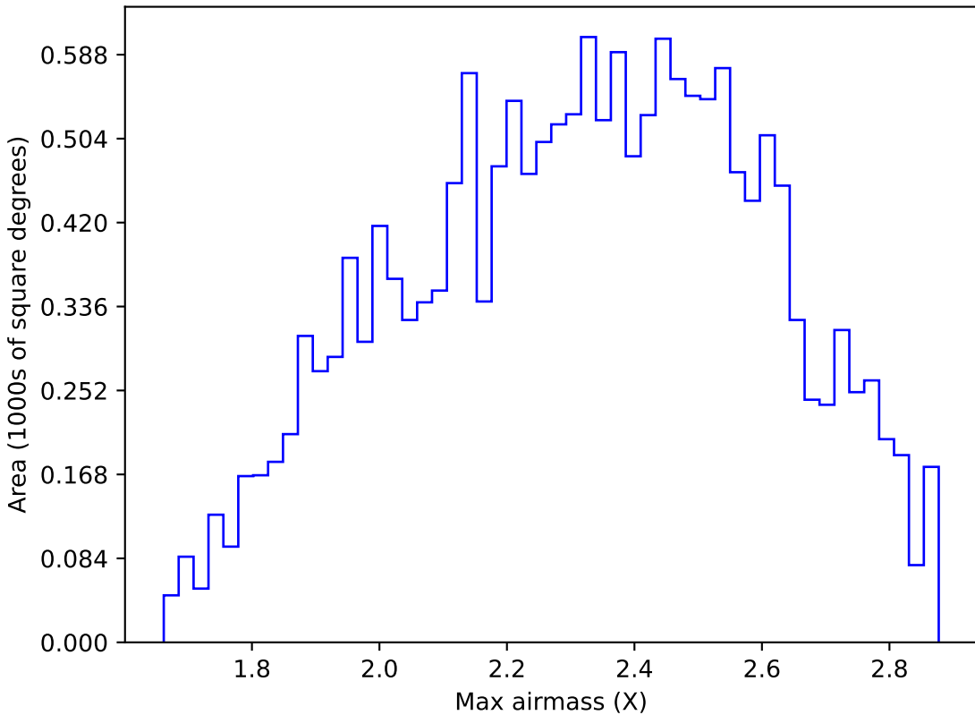
ddf_loaded_half_fl4_v3.4_10yrs WFD y band: Max airmass
