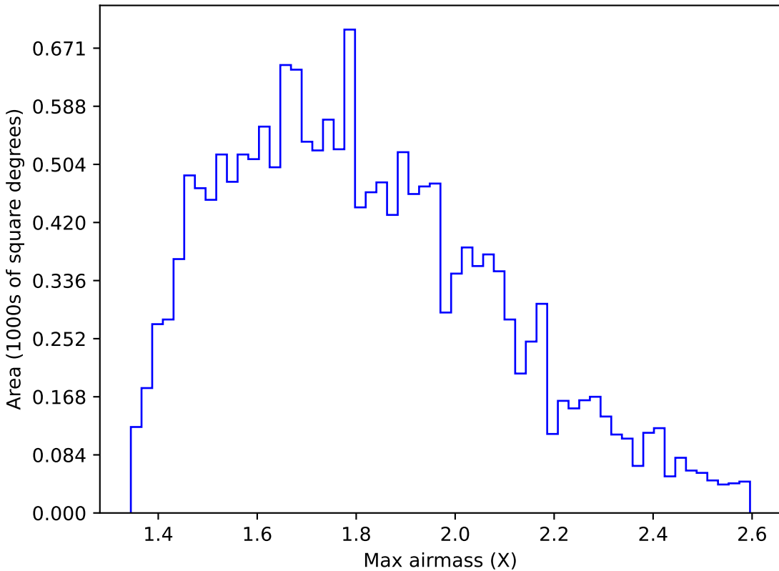
ddf_loaded_half_fl4_v3.4_10yrs WFD u band: Max airmass
