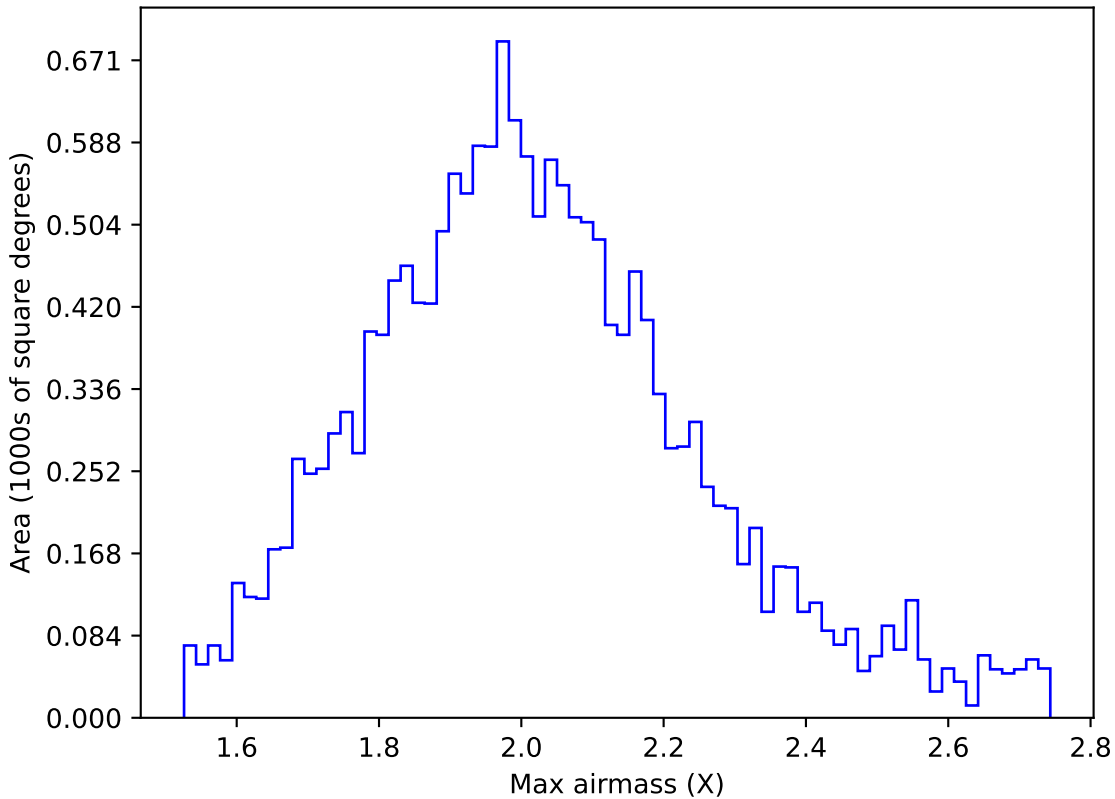
ddf_loaded_half_fl4_v3.4_10yrs WFD g band: Max airmass
