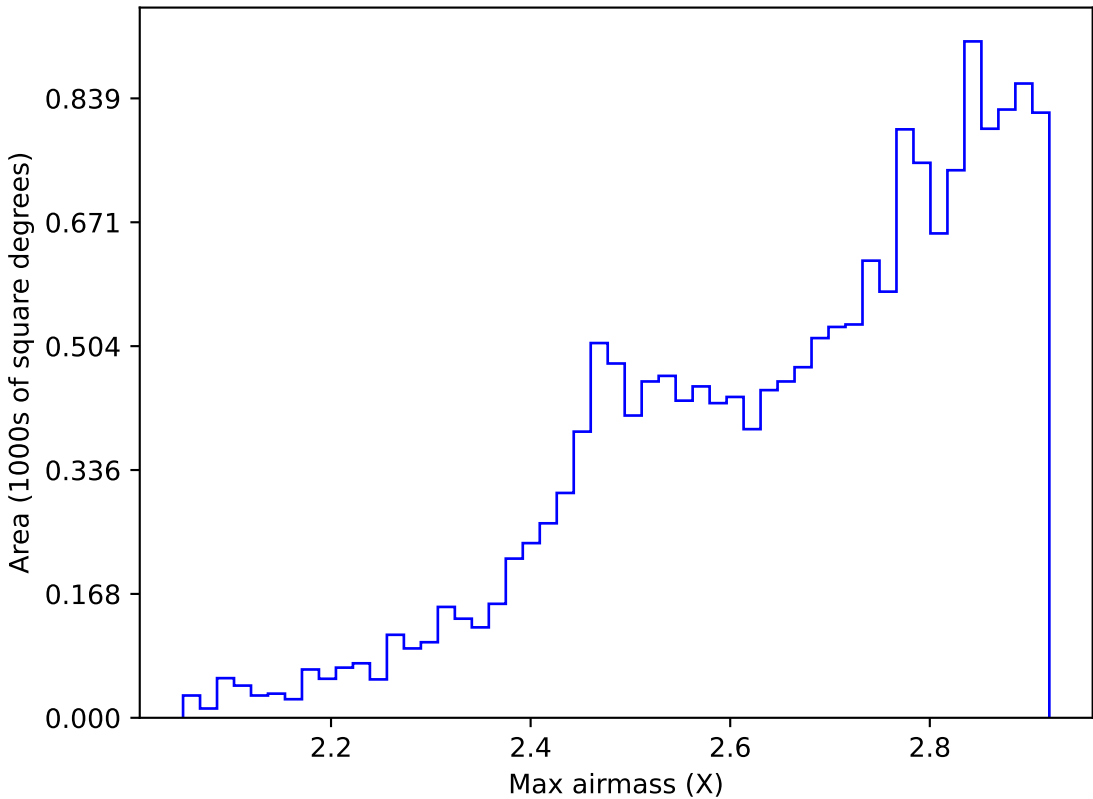
ddf_loaded_half_fl4_v3.4_10yrs WFD all bands: Max airmass
