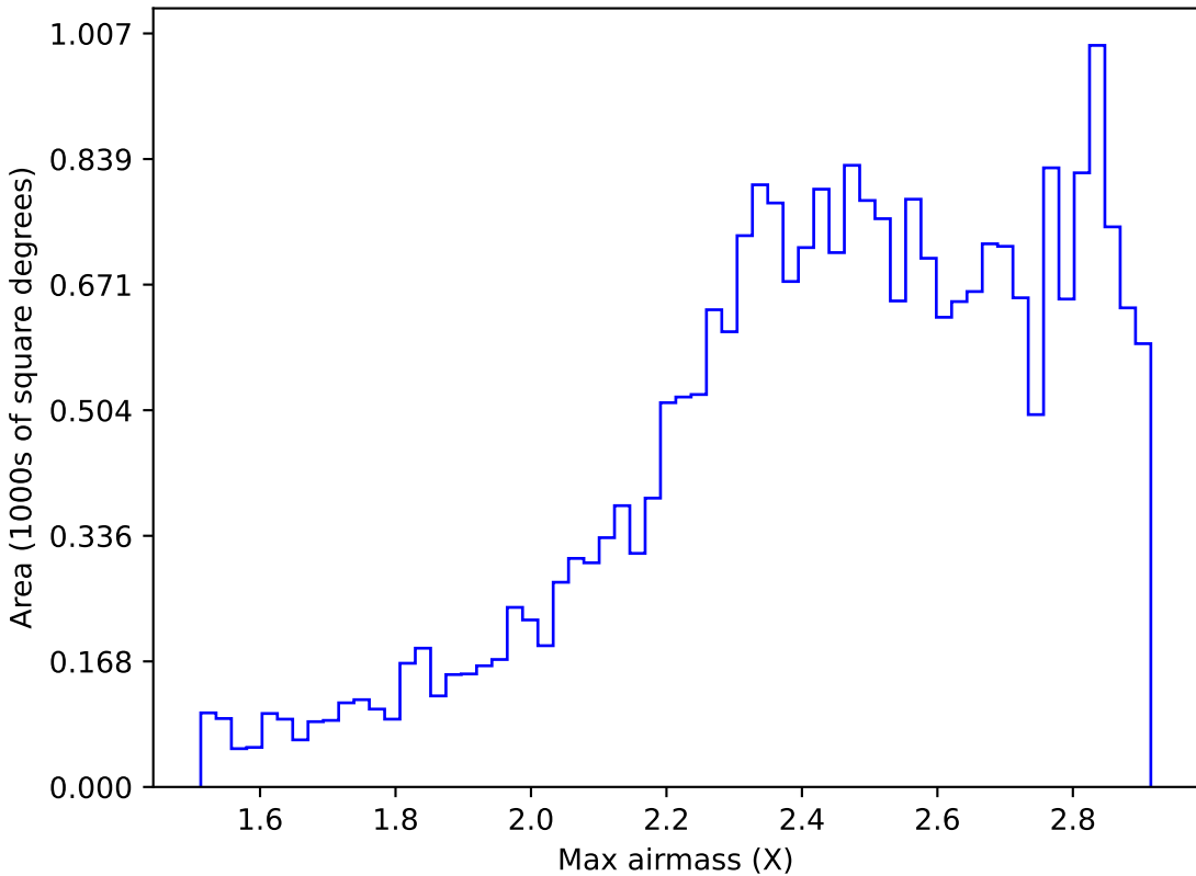
ddf_loaded_half_fl4_v3.4_10yrs All sky z band: Max airmass
