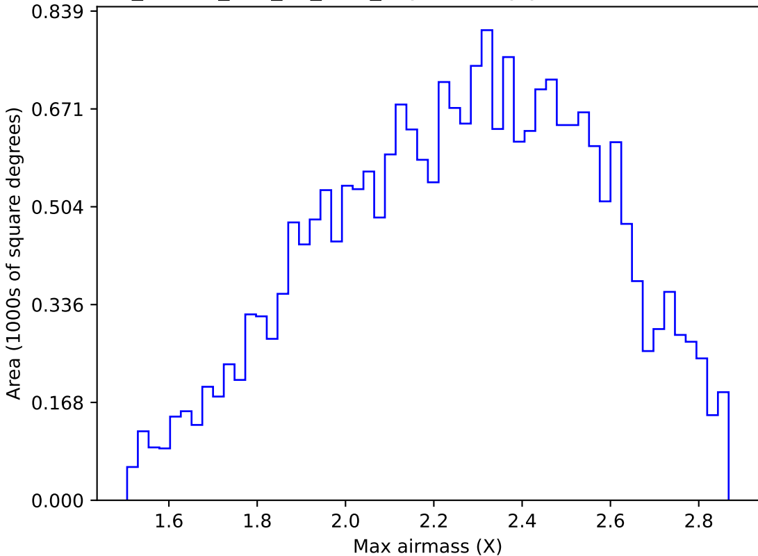
ddf_loaded_half_fl4_v3.4_10yrs All sky y band: Max airmass
