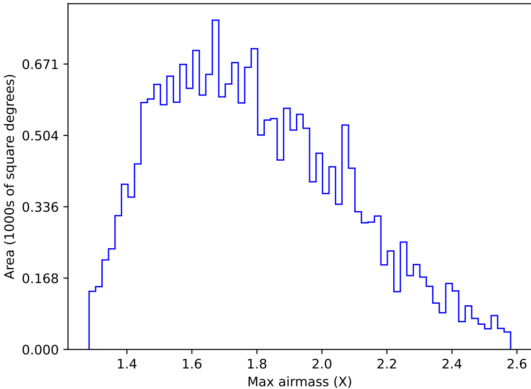
ddf_loaded_half_fl4_v3.4_10yrs All sky u band: Max airmass
