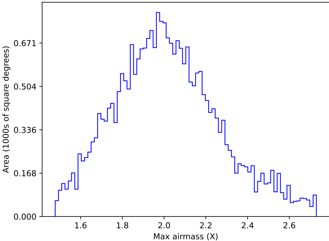
ddf_loaded_half_fl4_v3.4_10yrs All sky g band: Max airmass
