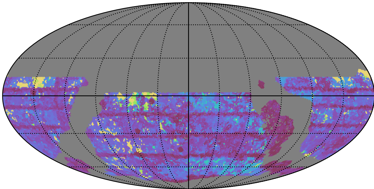
ddf_loaded_half_fl4_v3.4_10yrs WFD z band: Max Inter-Night Gap
