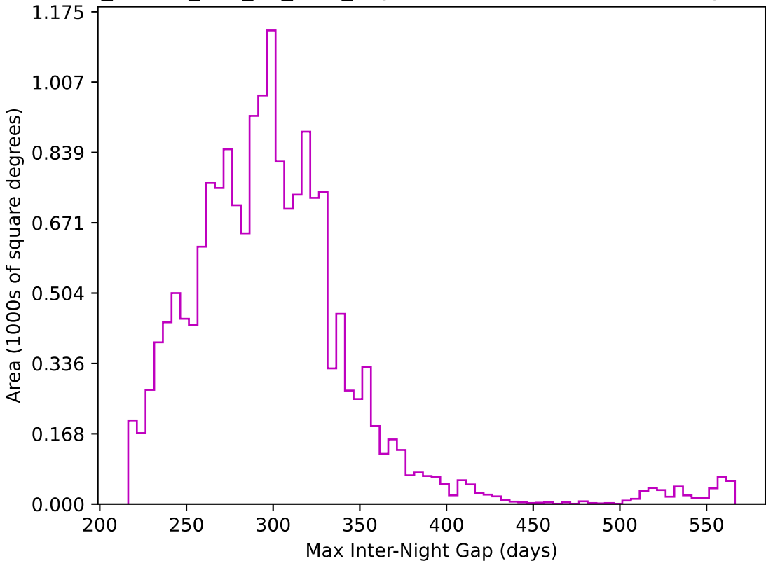
ddf_loaded_half_fl4_v3.4_10yrs WFD z band: Max Inter-Night Gap
