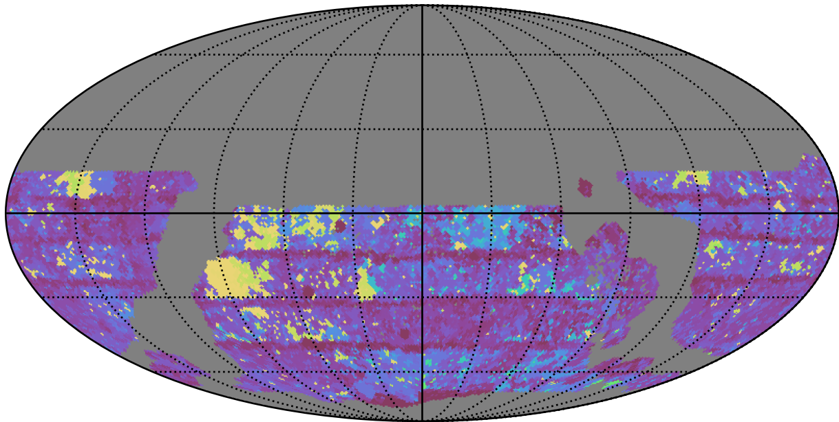
ddf_loaded_half_fl4_v3.4_10yrs WFD y band: Max Inter-Night Gap
