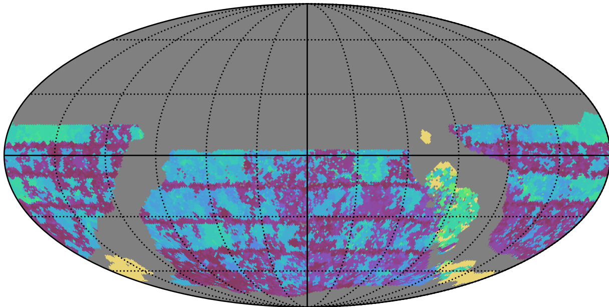
ddf_loaded_half_fl4_v3.4_10yrs WFD u band: Max Inter-Night Gap
