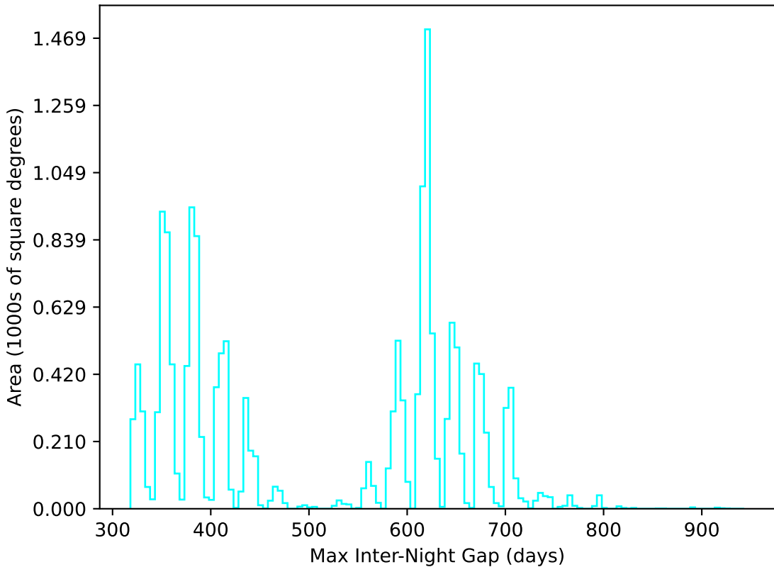
ddf_loaded_half_fl4_v3.4_10yrs WFD u band: Max Inter-Night Gap
