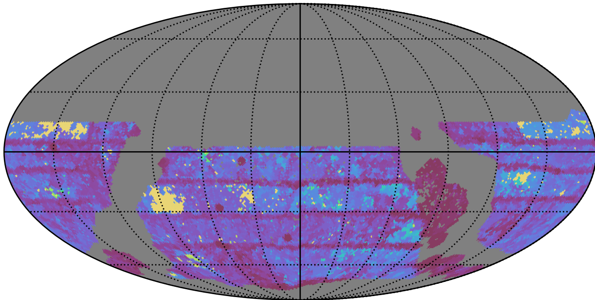
ddf_loaded_half_fl4_v3.4_10yrs WFD r band: Max Inter-Night Gap
