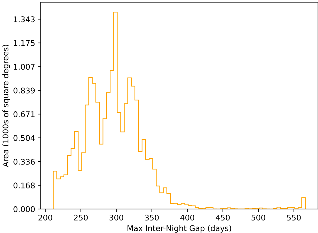
ddf_loaded_half_fl4_v3.4_10yrs WFD r band: Max Inter-Night Gap
