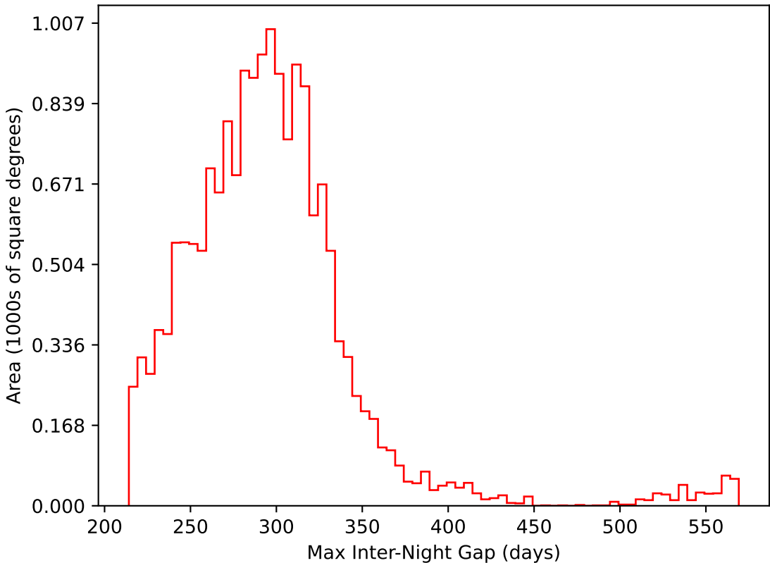
ddf_loaded_half_fl4_v3.4_10yrs WFD i band: Max Inter-Night Gap
