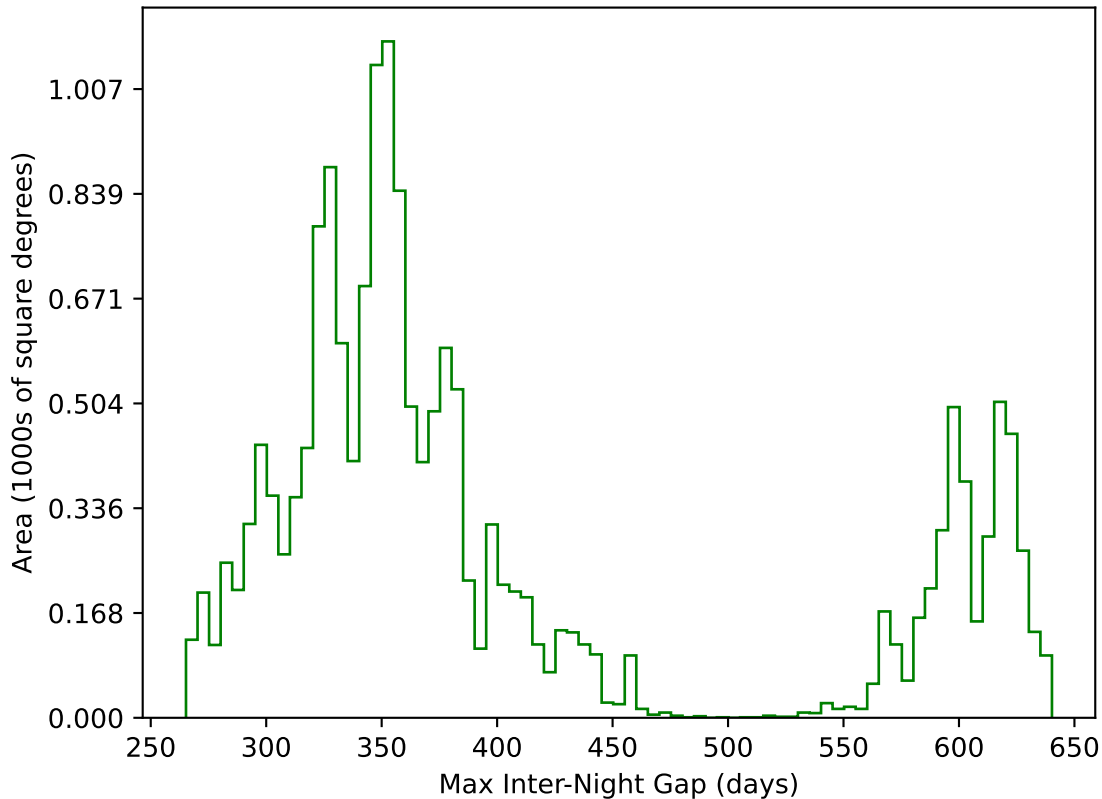
ddf_loaded_half_fl4_v3.4_10yrs WFD g band: Max Inter-Night Gap
