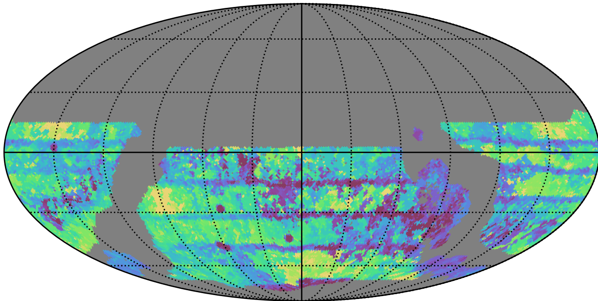
ddf_loaded_half_fl4_v3.4_10yrs WFD all bands: Max Inter-Night Gap
