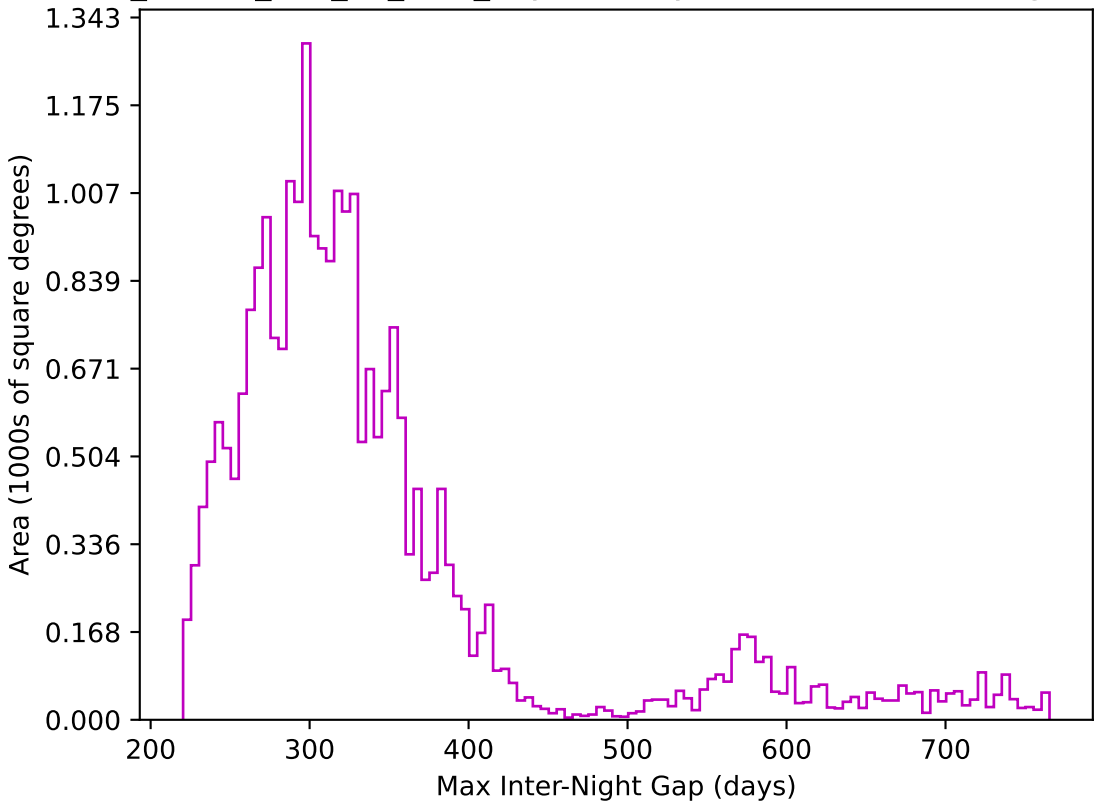
ddf_loaded_half_fl4_v3.4_10yrs All sky z band: Max Inter-Night Gap
