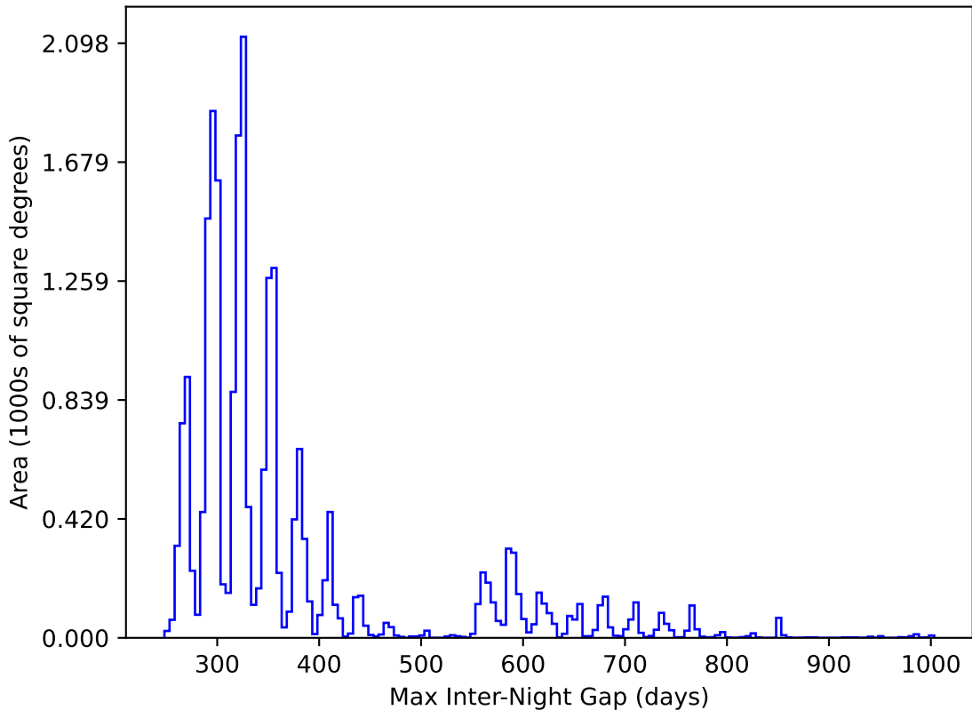
ddf_loaded_half_fl4_v3.4_10yrs All sky y band: Max Inter-Night Gap
