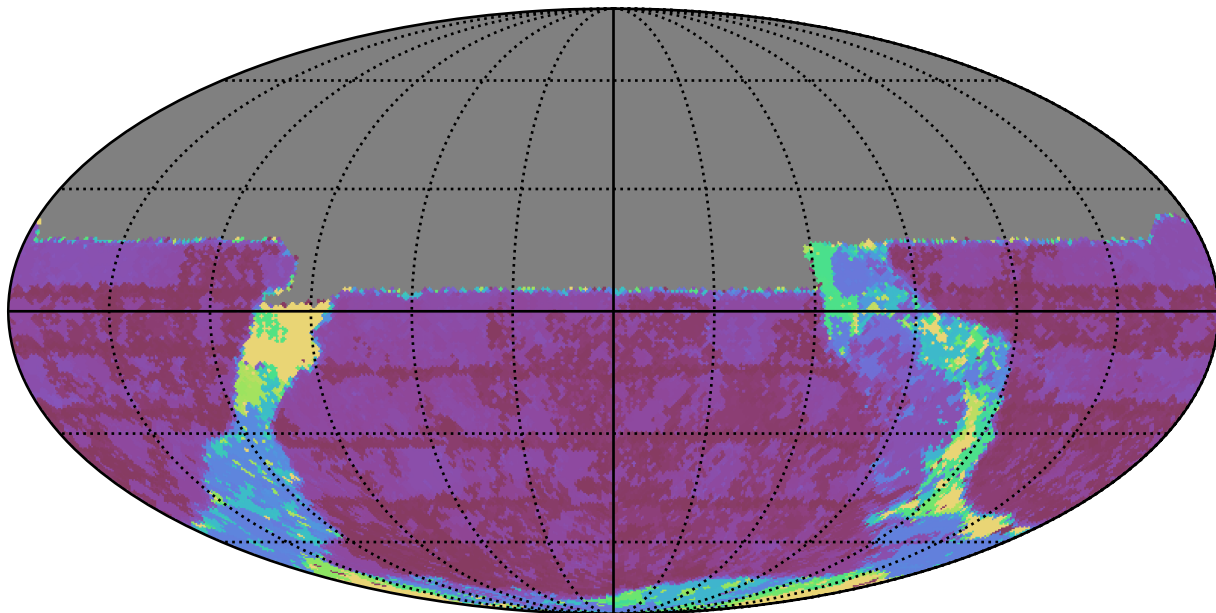
ddf_loaded_half_fl4_v3.4_10yrs All sky u band: Max Inter-Night Gap
