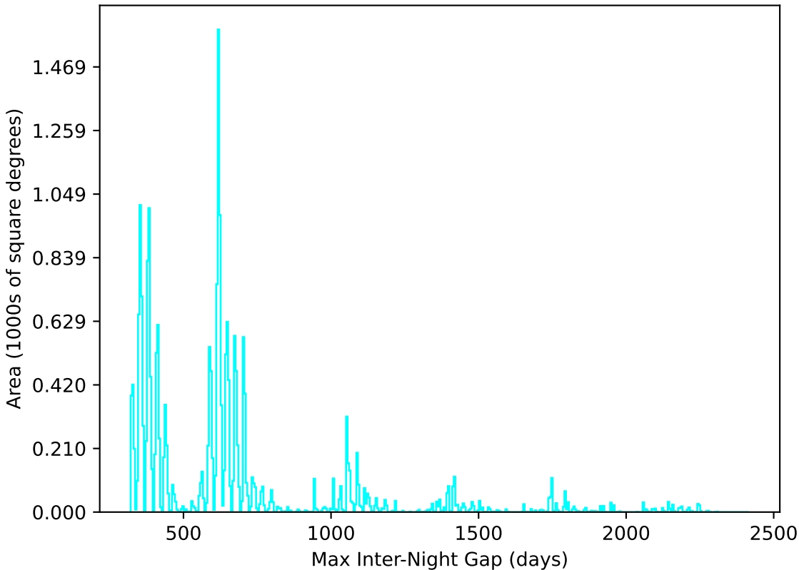
ddf_loaded_half_fl4_v3.4_10yrs All sky u band: Max Inter-Night Gap
