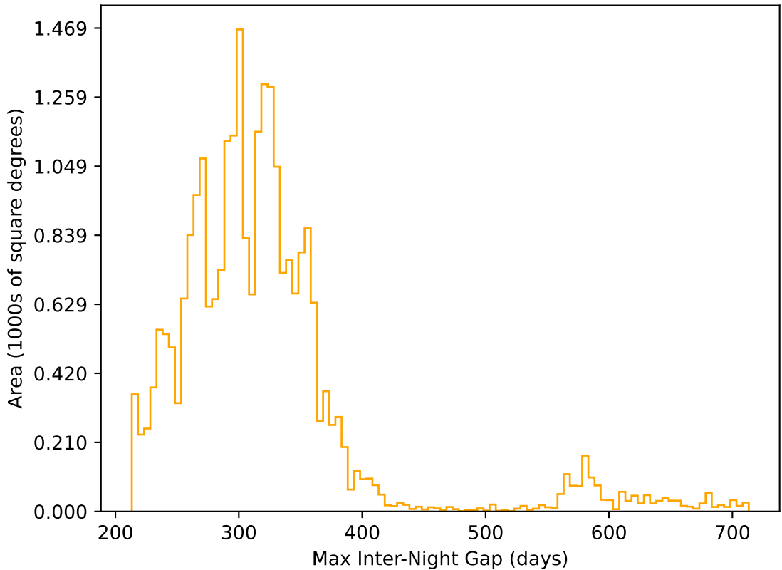
ddf_loaded_half_fl4_v3.4_10yrs All sky r band: Max Inter-Night Gap
