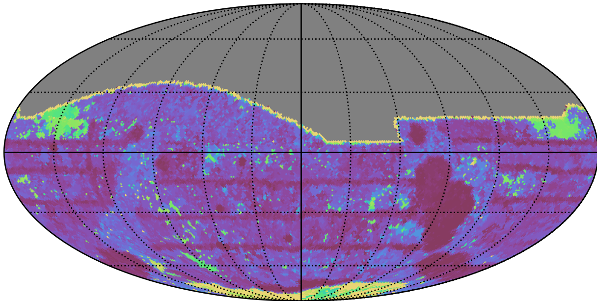
ddf_loaded_half_fl4_v3.4_10yrs All sky i band: Max Inter-Night Gap
