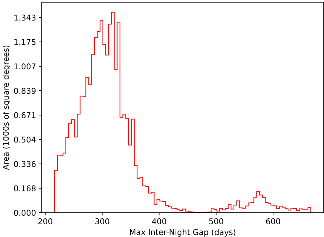
ddf_loaded_half_fl4_v3.4_10yrs All sky i band: Max Inter-Night Gap
