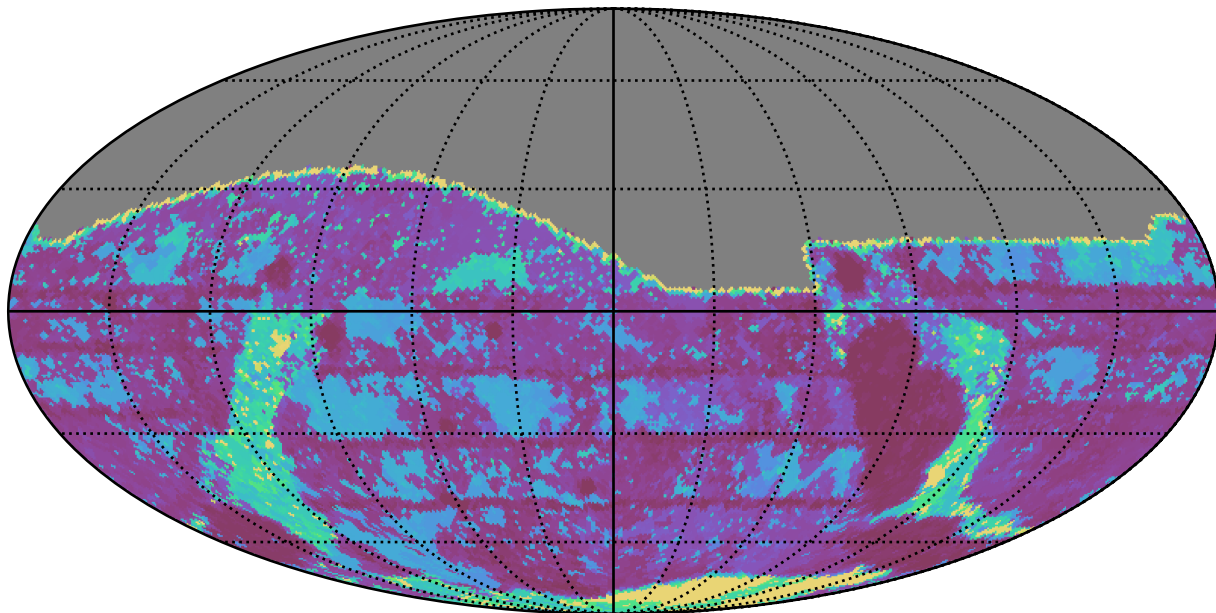
ddf_loaded_half_fl4_v3.4_10yrs All sky g band: Max Inter-Night Gap
