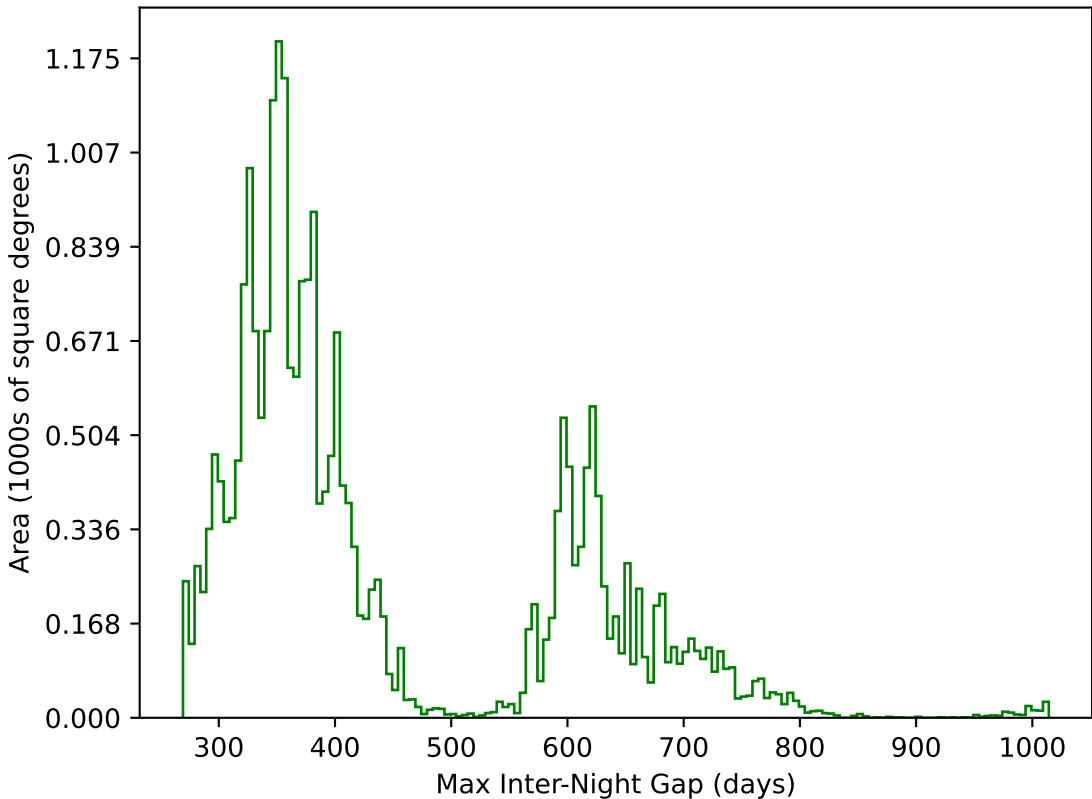
ddf_loaded_half_fl4_v3.4_10yrs All sky g band: Max Inter-Night Gap
