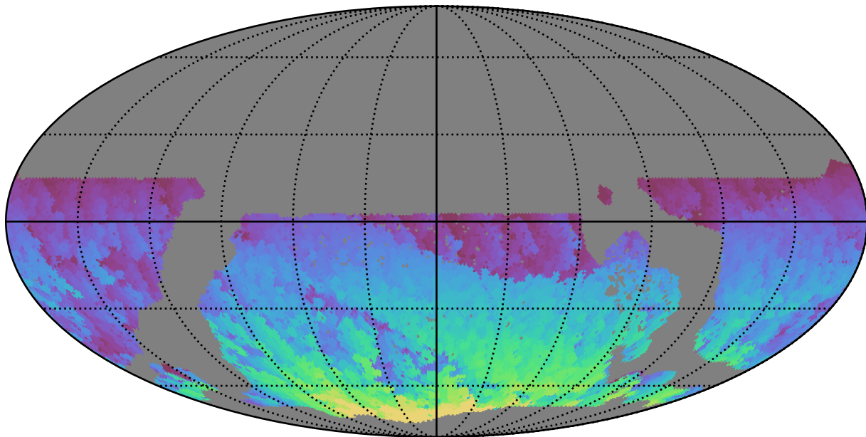
ddf_loaded_half_fl4_v3.4_10yrs WFD z band: Max HA
