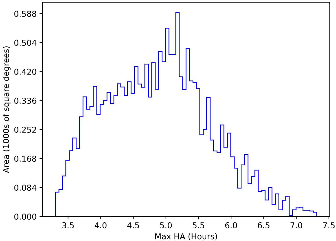
ddf_loaded_half_fl4_v3.4_10yrs WFD z band: Max HA
