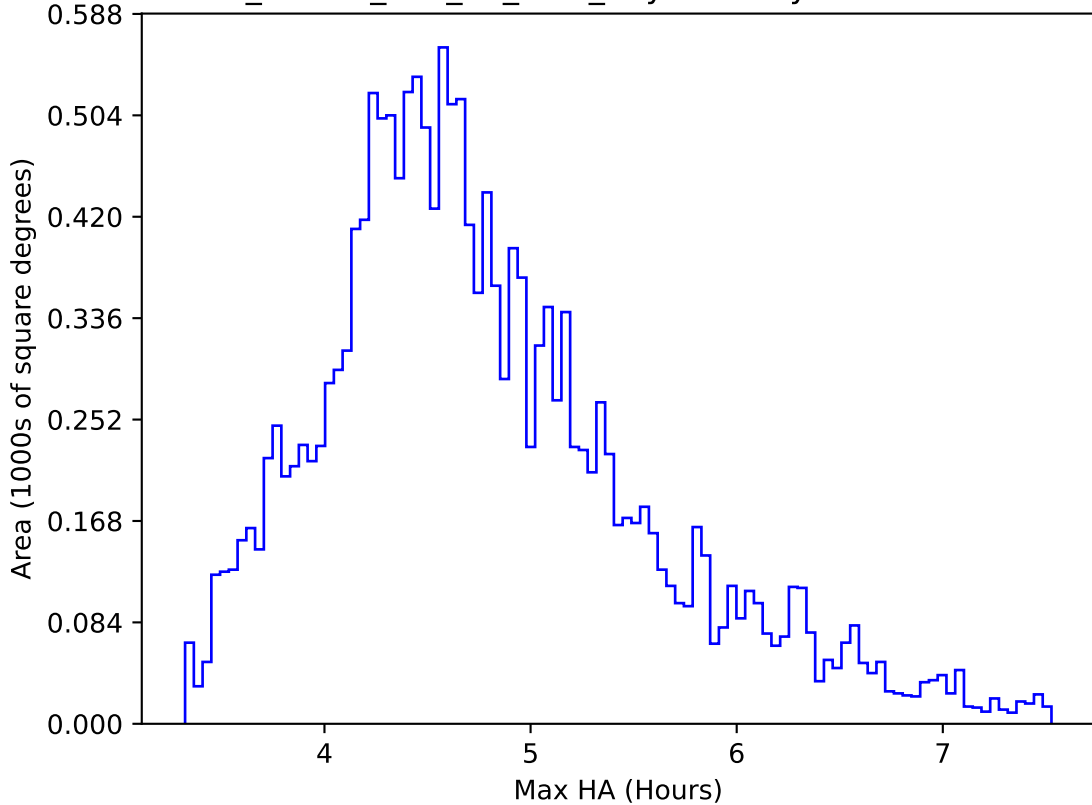
ddf_loaded_half_fl4_v3.4_10yrs WFD y band: Max HA
