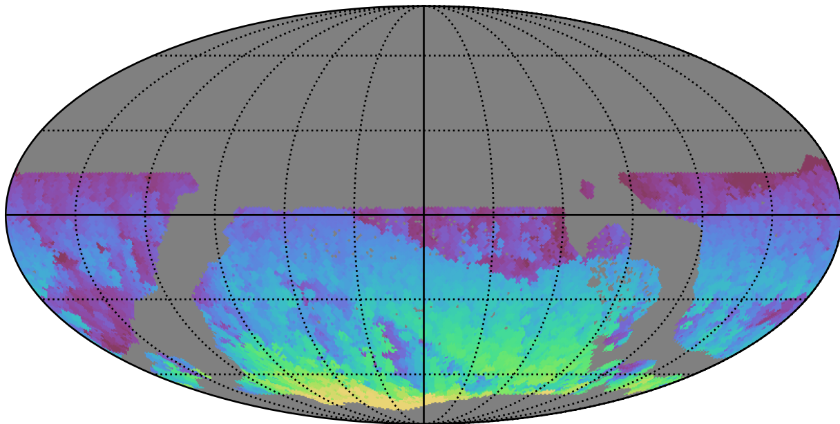
ddf_loaded_half_fl4_v3.4_10yrs WFD i band: Max HA
