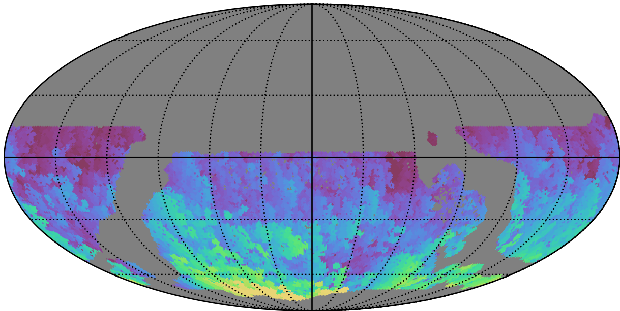
ddf_loaded_half_fl4_v3.4_10yrs WFD g band: Max HA
