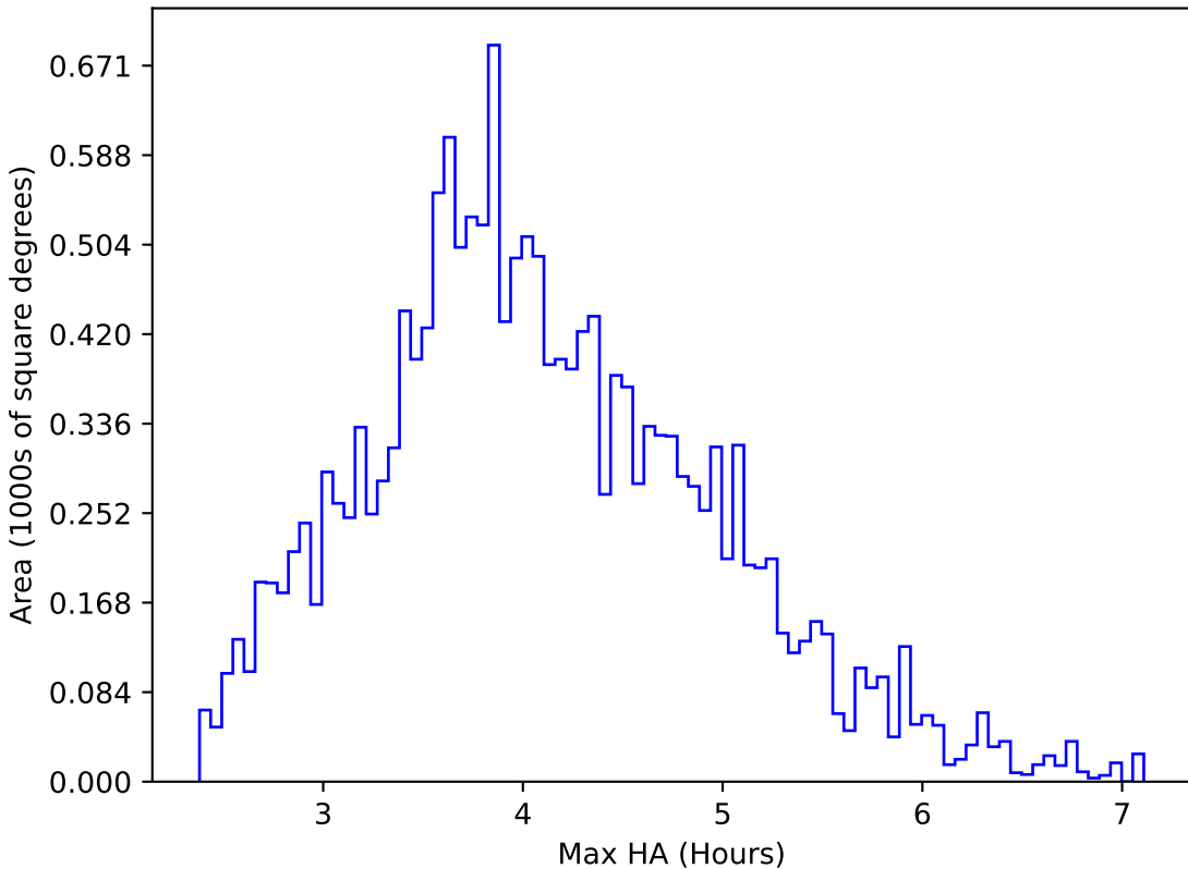
ddf_loaded_half_fl4_v3.4_10yrs WFD g band: Max HA
