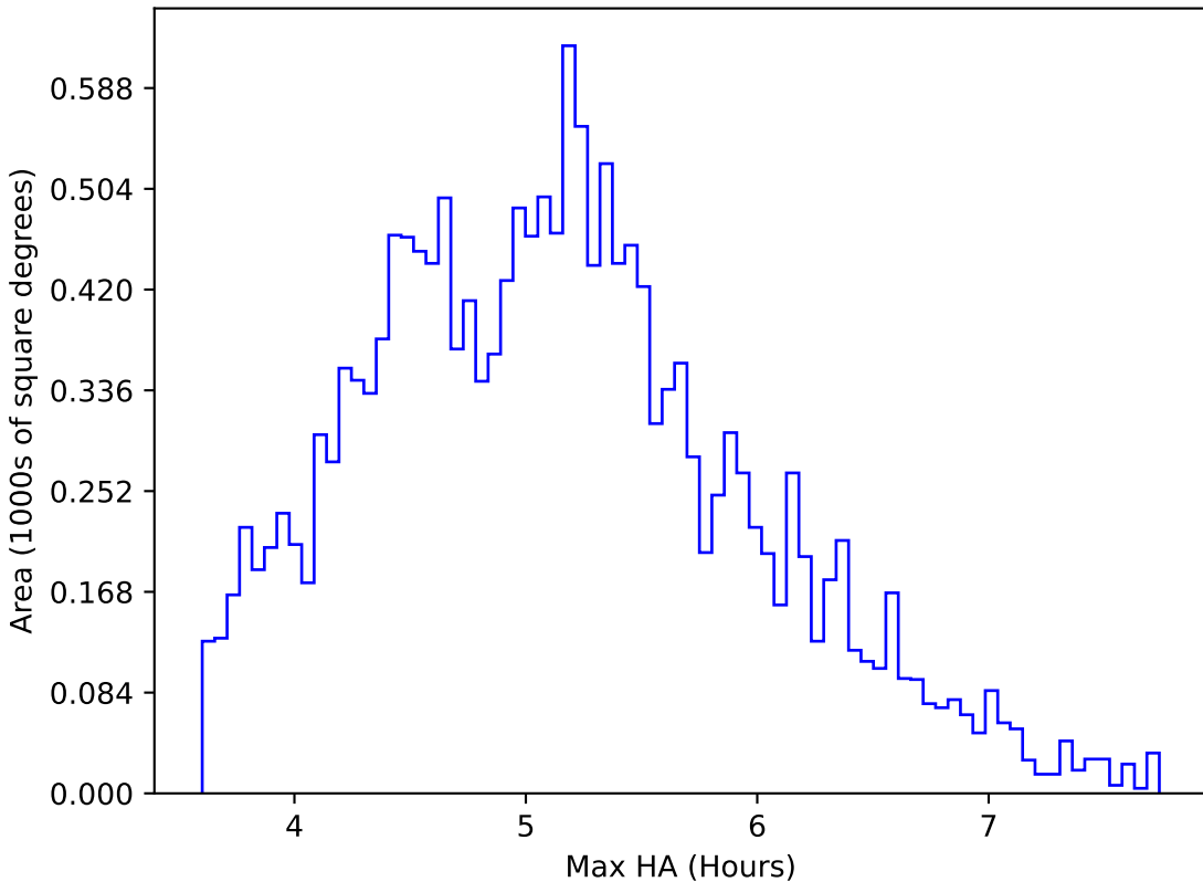
ddf_loaded_half_fl4_v3.4_10yrs WFD all bands: Max HA
