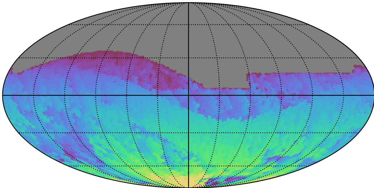
ddf_loaded_half_fl4_v3.4_10yrs All sky z band: Max HA
