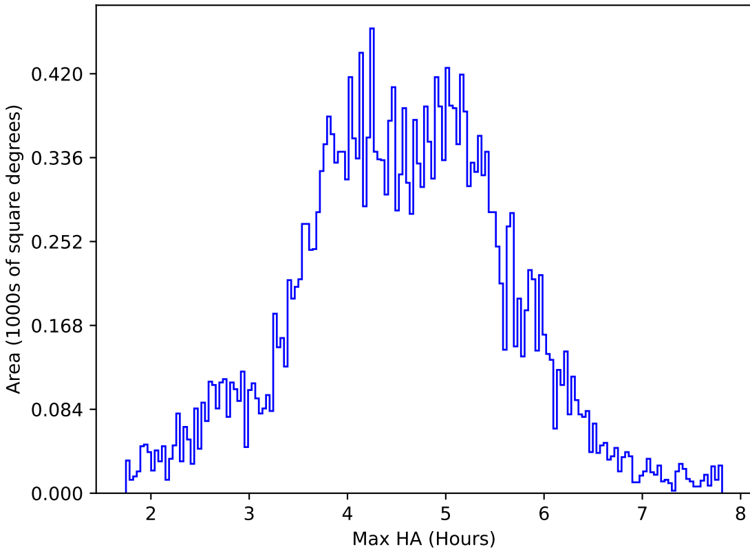
ddf_loaded_half_fl4_v3.4_10yrs All sky z band: Max HA
