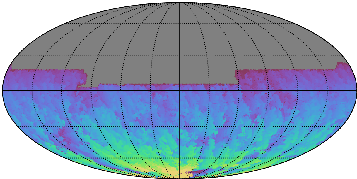
ddf_loaded_half_fl4_v3.4_10yrs All sky y band: Max HA
