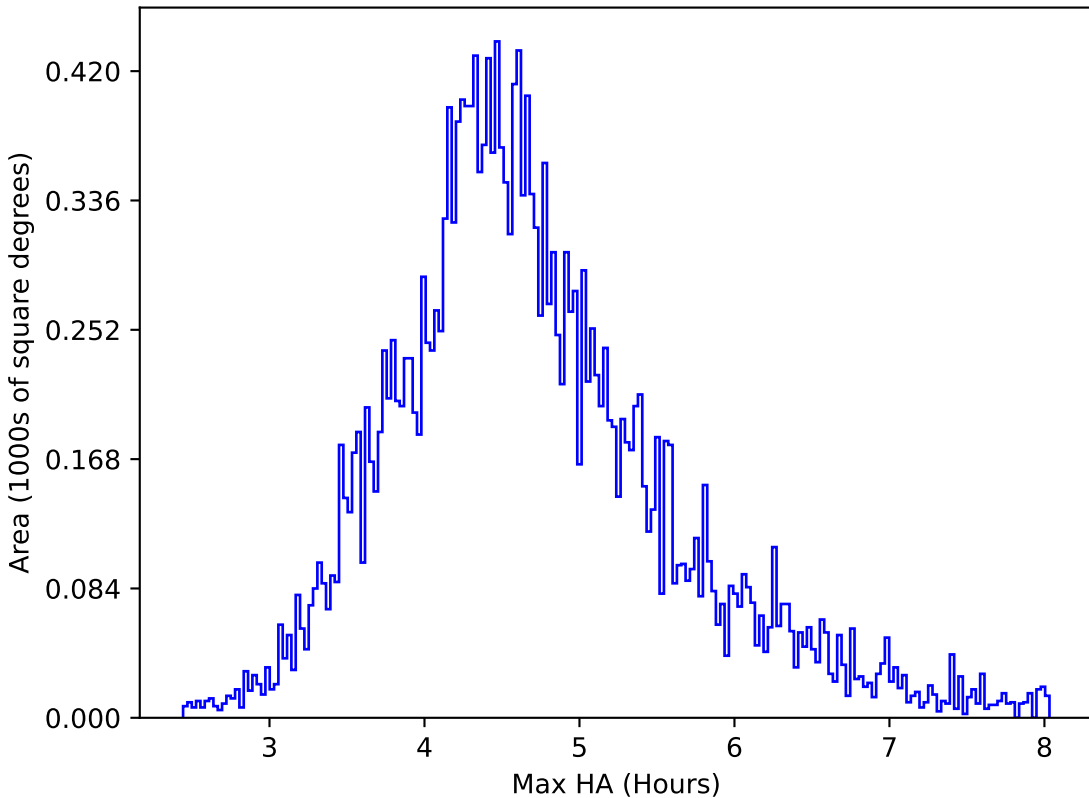
ddf_loaded_half_fl4_v3.4_10yrs All sky y band: Max HA
