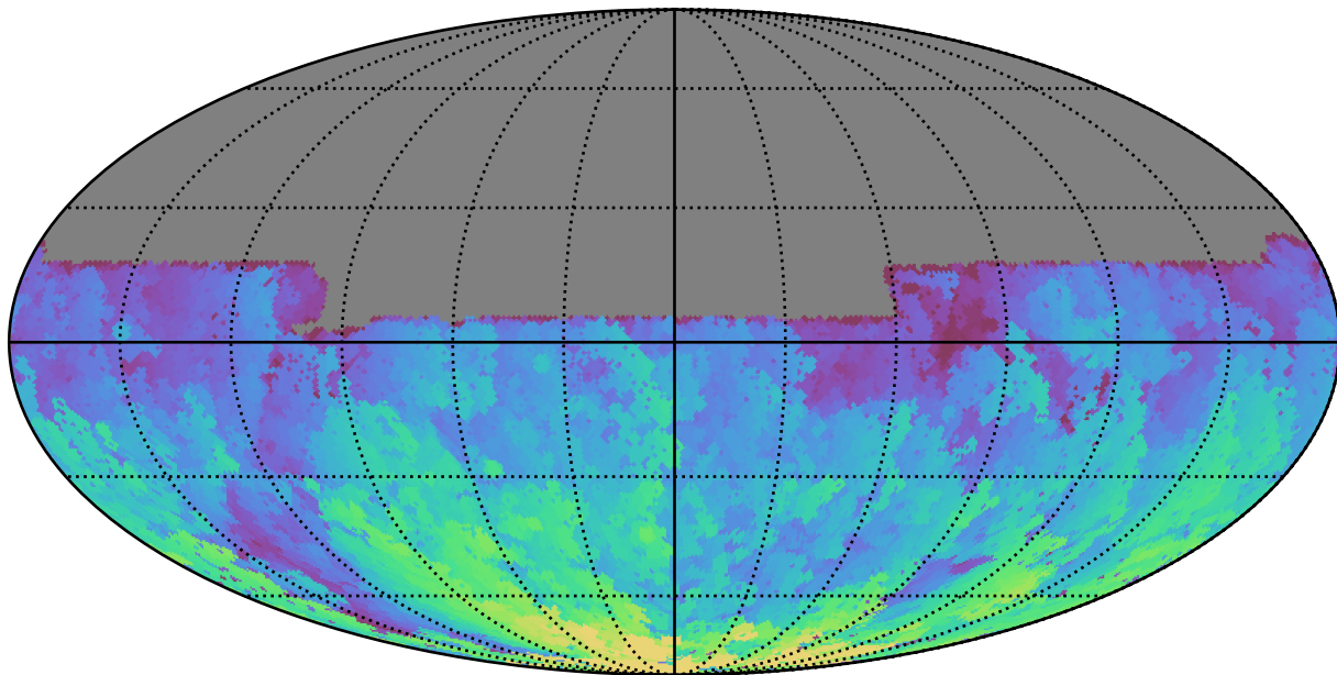
ddf_loaded_half_fl4_v3.4_10yrs All sky u band: Max HA
