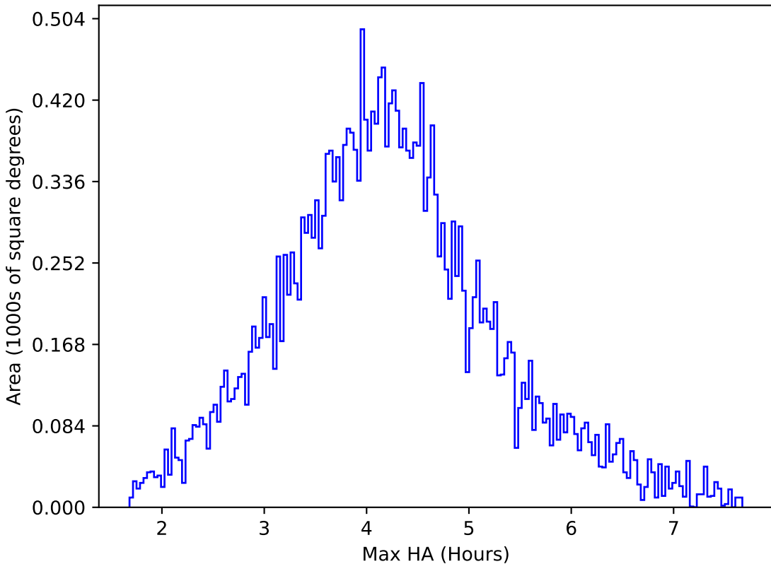
ddf_loaded_half_fl4_v3.4_10yrs All sky r band: Max HA
