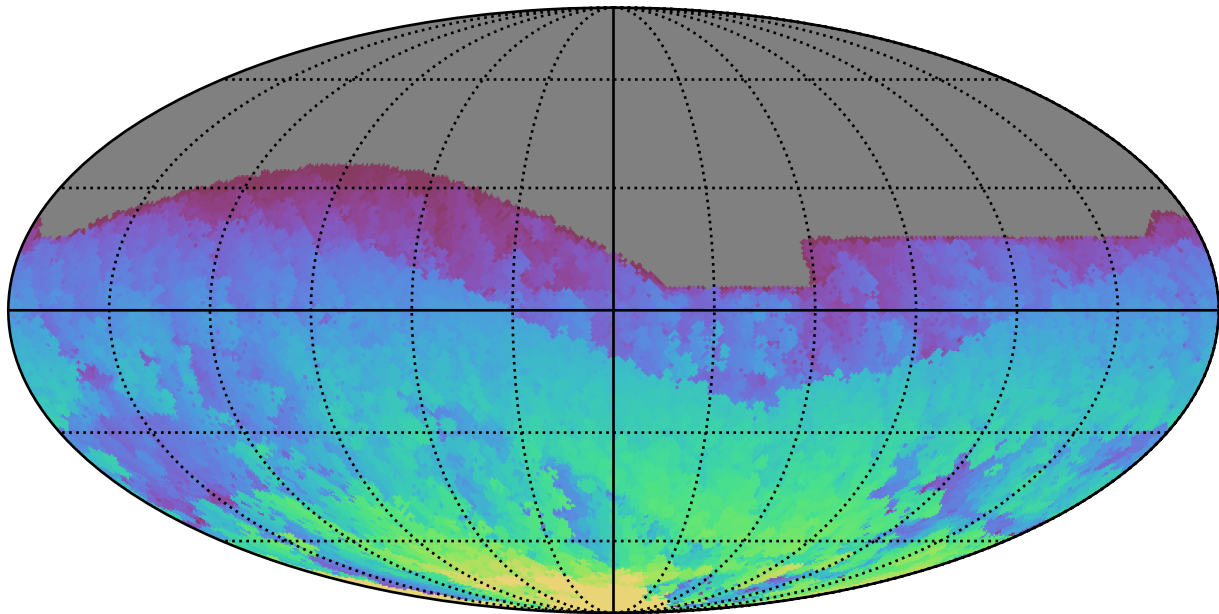
ddf_loaded_half_fl4_v3.4_10yrs All sky i band: Max HA
