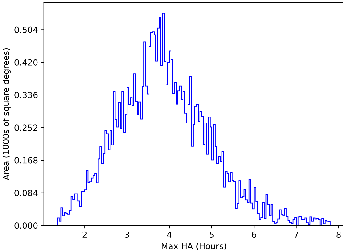
ddf_loaded_half_fl4_v3.4_10yrs All sky g band: Max HA
