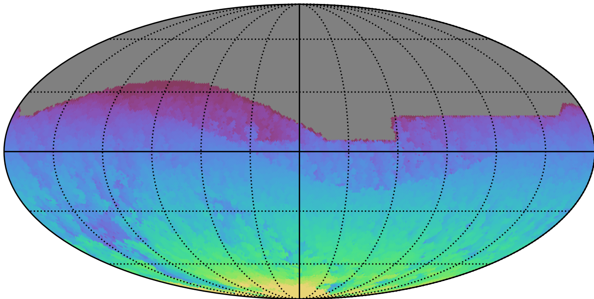
ddf_loaded_half_fl4_v3.4_10yrs All sky all bands: Max HA
