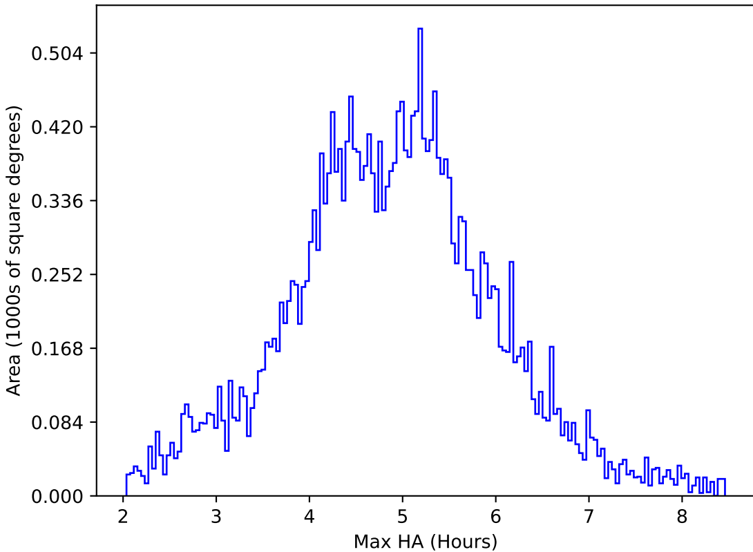
ddf_loaded_half_fl4_v3.4_10yrs All sky all bands: Max HA
