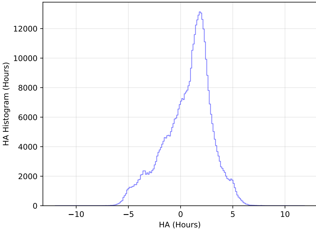
ddf_loaded_half_fl4_v3.4_10yrs WFD z band: HA Histogram
